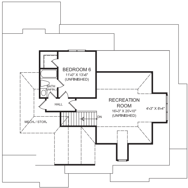
THIRD FLOOR
